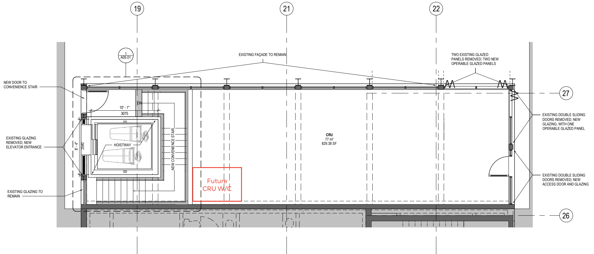
1 CONSTRUCTION PLAN - LEVEL 01 SCALE: 1/4" = 1'-0"
