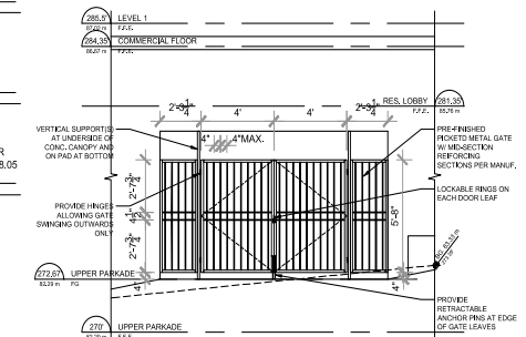
2 GAS METER GATE AT LANE A4.02 1/4"= 1'-0"
