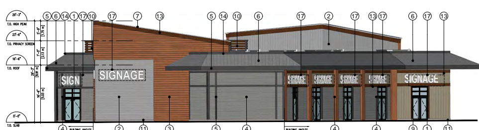
2 SOUTH ELEVATION ADD 1/8"=1'-0"
