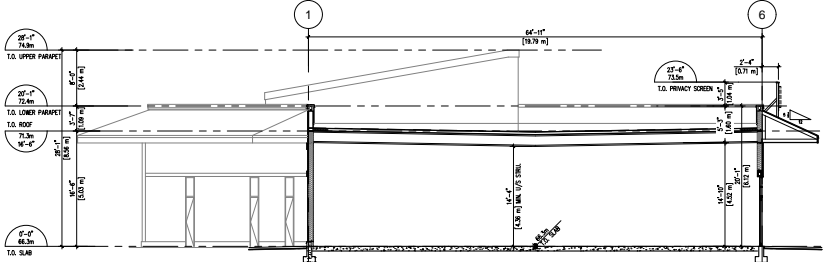
5 BUILDING SECTION ADD 1/8"=1'-0"
